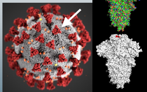
Computational Modeling
